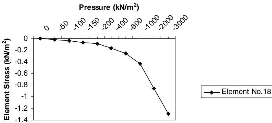
Fig.5 Pressure vs Element Stress (Sigx) Curve
